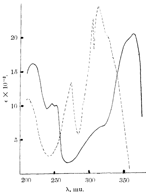
Fig. 2.—Ultraviolet light absorption of ethyl 4-imino-8-methyl-4H-pyrido[1,2-a]pyrimidine-3-carboxylate (----) and 3-cyano-2-keto-2H-pyrido[1,2-a]pyrimidine (—).
